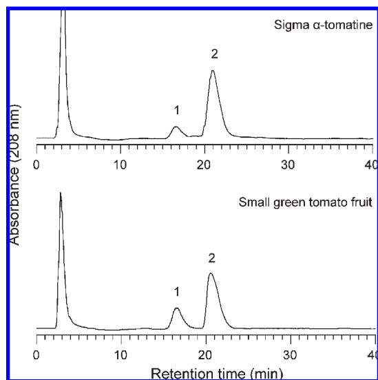
Figure 2. HPLC chromatograms of standard Sigma tomatine and an extract from a small green tomato: column, Inertsil NH 2 (5 \mu m, 4.0 \times 250 mm); column temperature, 30 ^{\circ} C; mobile phase, acetonitrile/20 mM KH 2 PO 4 (23:77, v/v); flow rate, 1 mL/min. Peaks: 1, dehydrotomatine; 2, \alpha -tomatine.
